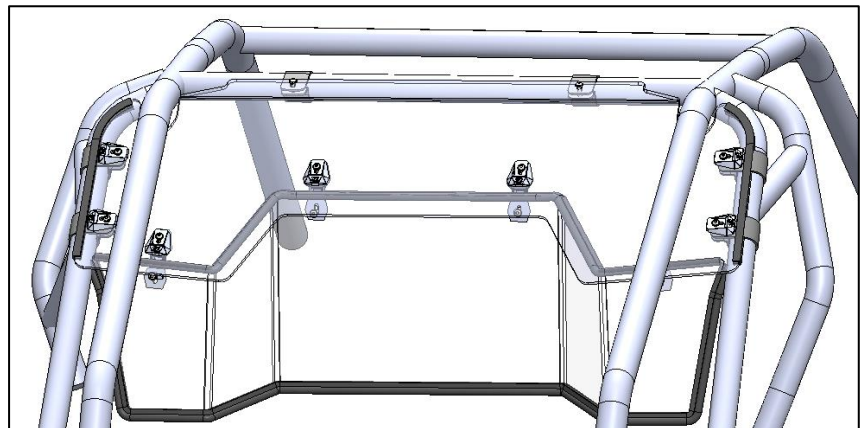
12. The bracket slots allow for adjustment in the lower windshield so that you may ensure the windshield gasket seals along bottom edge. Make sure windshield is centered and snug, tighten all bolts.
