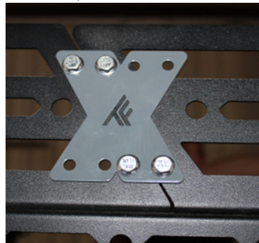
FIG 17 - Fasten together Upper Rack - FRONT and Upper Rack - REAR using 10mm Socket and 10mm Wrench
