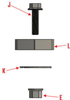
FIG 5 - Using 7/16" Socket & 7/16" Wrench Install Washers to Front Corners of Bed
