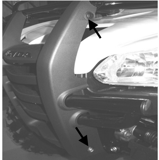
Figure 1 Remove front Plastic Bumper Cover
