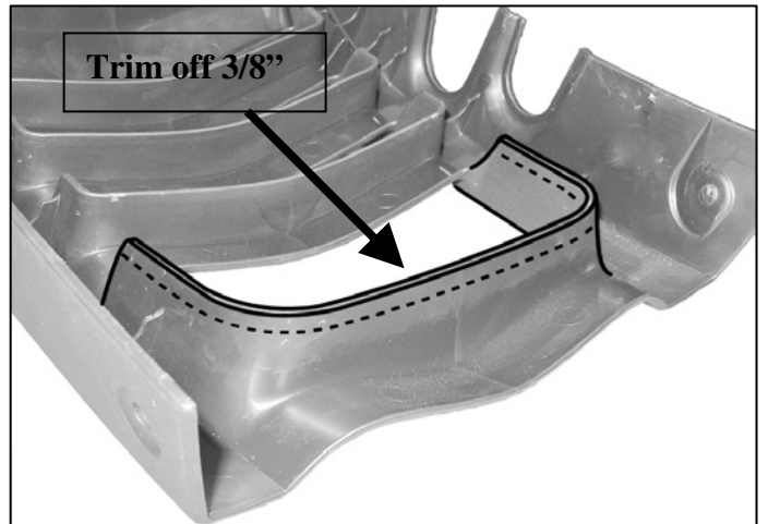
Figure 7 - Trim Bumper Cover
