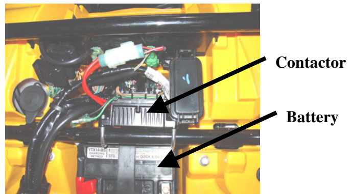
Figure 8 Contactor & Battery
