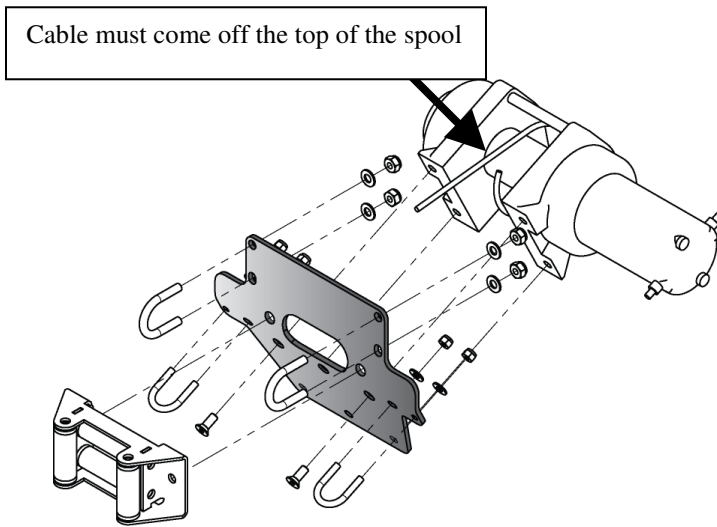
Figure 5 4-Hole mounted Winch
