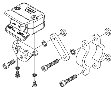
Figure 6: Mini-rocker switch assembly.
