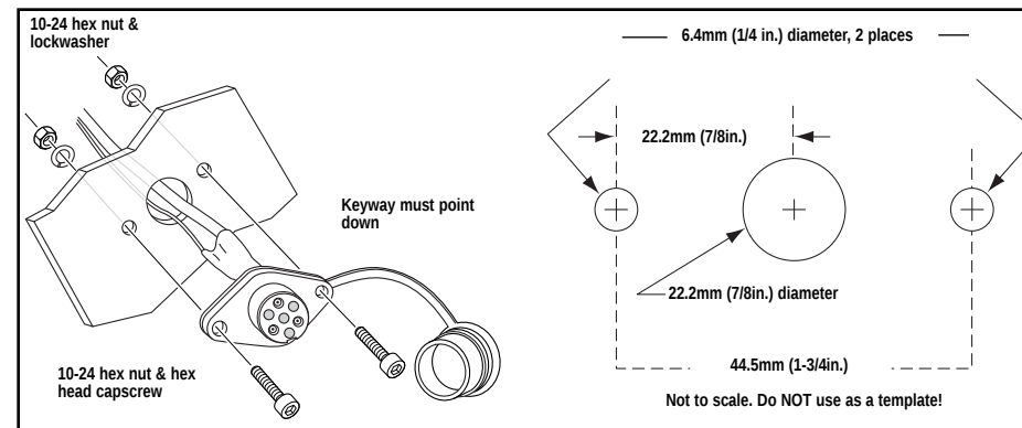
Figure 7 and 8. Remote socket installation
