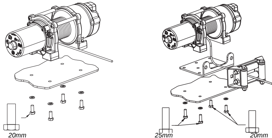
Figure 2 and 3: Orientation of winch to mounting plate and bolt lengths.
