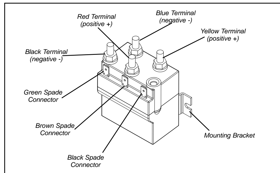
Figure 4. Contactor for the WARN ATV/UTV winch
