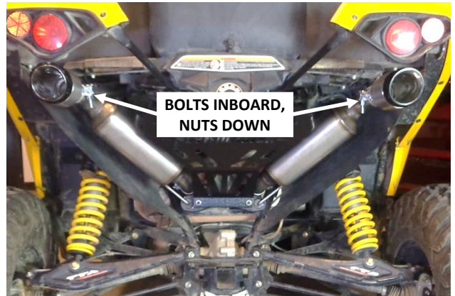
15. Note that, at Step 17, the tip clamps will be installed with the bolts inboard and the nuts pointed down.
