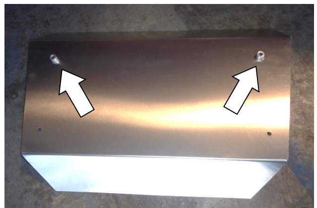
12. Place the heat shield backer (2) on a bench or other flat surface. Place spacers (7) over the top two holes.
