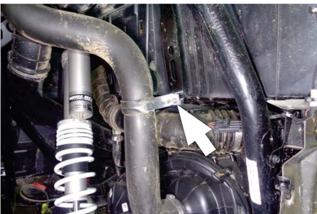
15. In the left rear wheel well, remove the bolt securing the clutch cooling air duct clamp to the frame.
