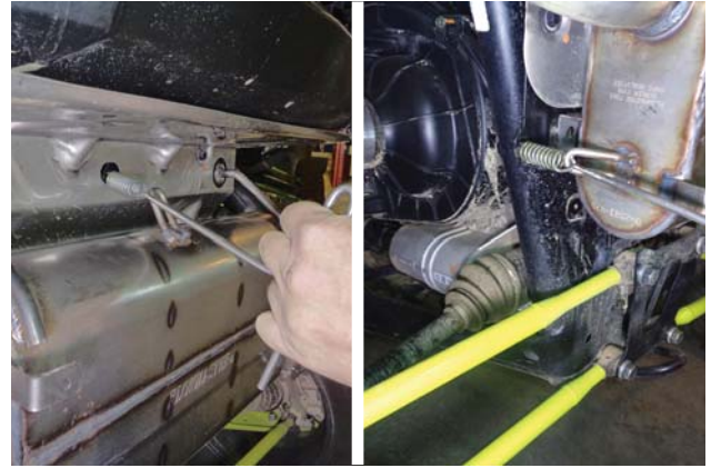
22. Use a spring puller to connect the 2 muffer mount springs to the muffer.
