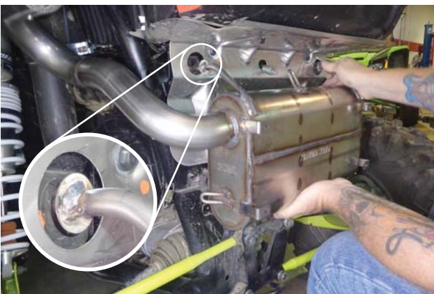
21. Install the muffer by pushing the hanger pins all the way into their rubber mounts. Verify proper alignment of the exhaust pipe and muffer flange.
